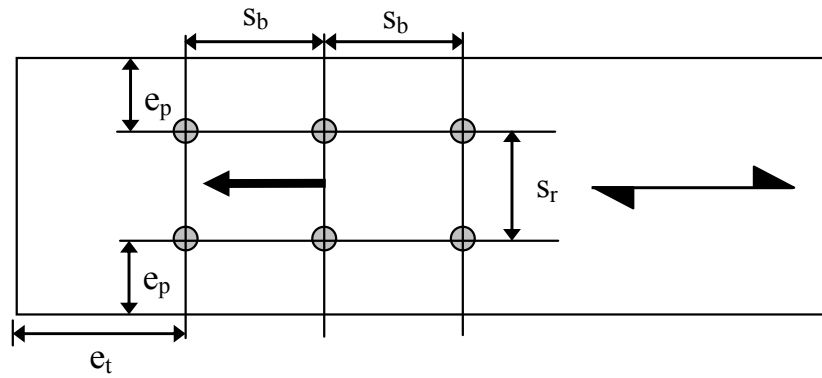
Figure 2. Nomenclature of the connections configuration variables parallel-to-grain
