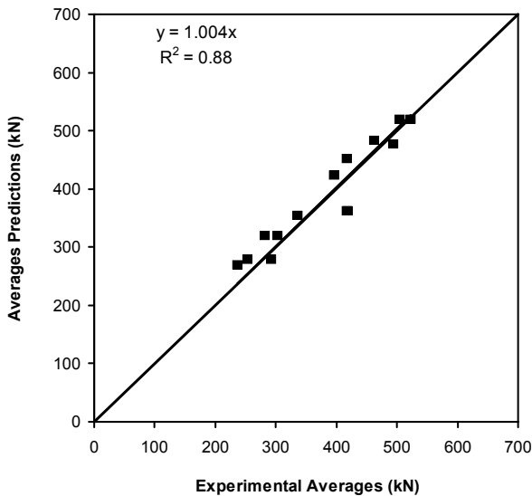
Figure 5. Predicted averages of connection capacity vs. experimental resistance averages in group tear-out failure mode
