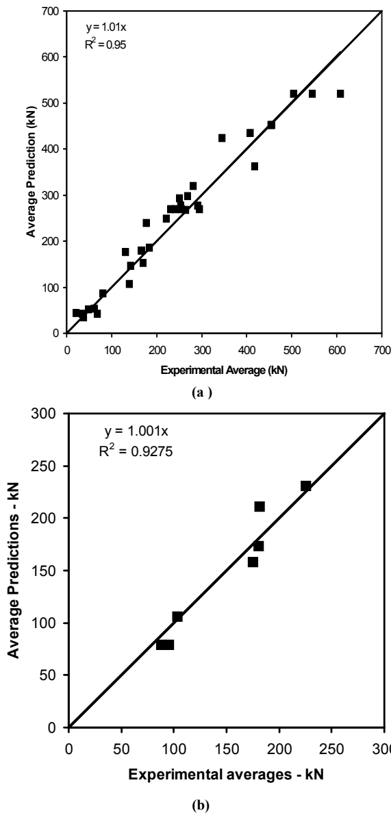
Figure 4. Predicted averages of connection capacity vs. experimental resistance average in row shear failure mode (a) steel-wood-steel connections (b) wood-steel-wood connections
