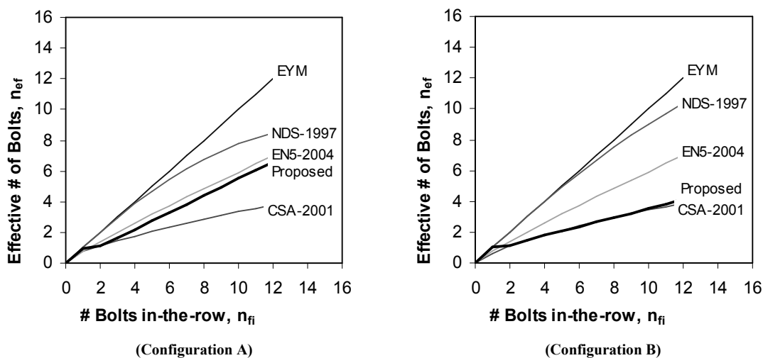
Figure 7. Comparison of the effective number of in-row bolts vs. the number of in-row bolts for various existing standards and the proposed design approach
