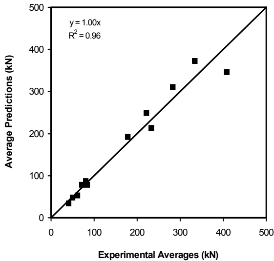
Figure 3. Predicted averages of connection capacity vs. experimental resistance averages in bearing failure mode
