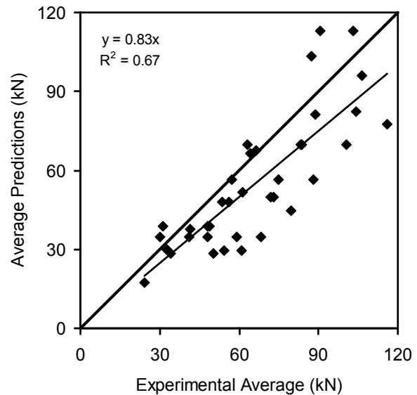
Figure 6. Predicted averages of connection capacity vs. experimental resistance averages bearing and splitting failures – connections loaded perpendicular-to-grain
