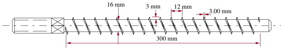
Screw A
