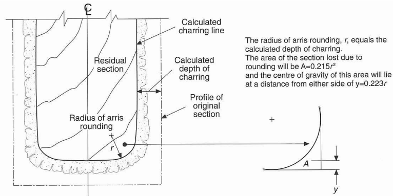
Figure 3. Definition of uncharred section area (15).
