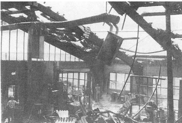
Figure 4. Unprotected glulam portal frame warehouse after a fire (15).
