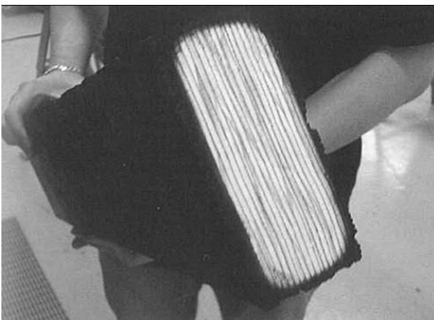
Figure 2. A charred section of LVL showing solid wood inside (5).
