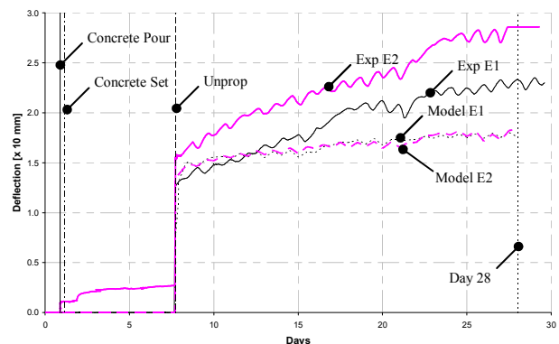
Figure 8. Experimental-numerical mid-span deflection comparison for indoor beams
