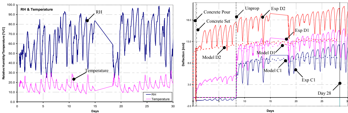
Figure 7. Experimental-numerical mid-span deflection comparison for outdoor beams (right) with corresponding relative humidity and temperature histories
