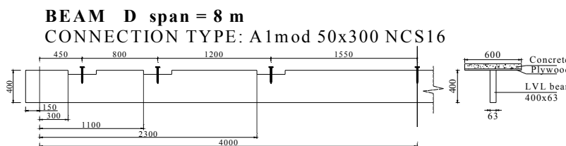
Figure 4. A typical 8 m TCC T-strip beam with a 300 mm length rectangular notched connection
