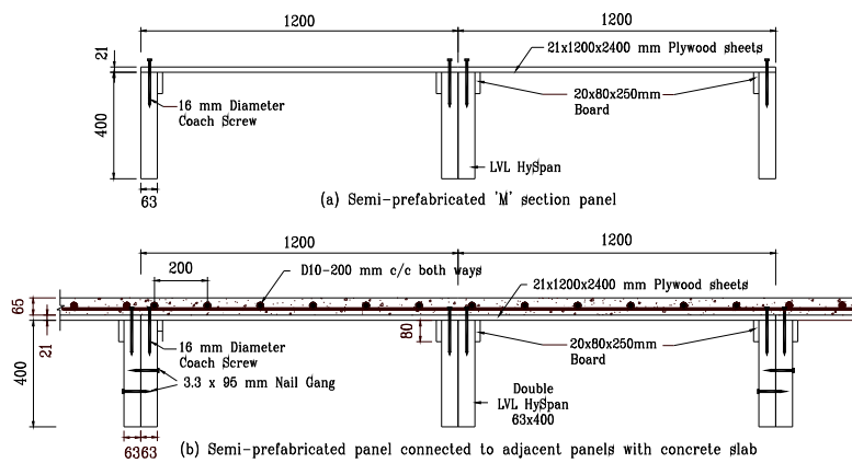
Figure 3. Semi-prefabricated “M” section panel (dimensions in mm)
