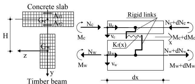
Figure 6. Cross-section (left) and elevation (right) of the uniaxial FE model used in the numerical analyses
