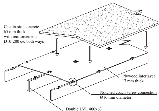
Figure 1. Proposed semi-prefabricated TCC floor system
