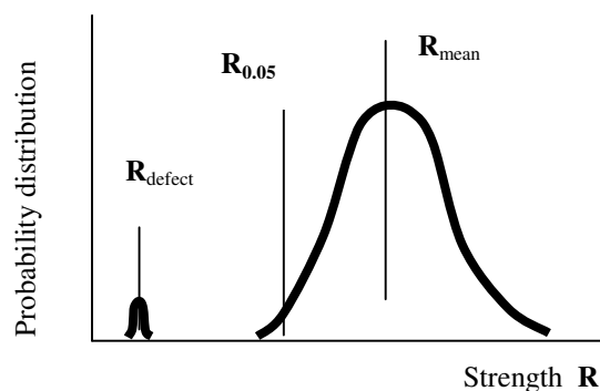
Figure 1. Schematic illustration of the strength distribution of a timber based element.
