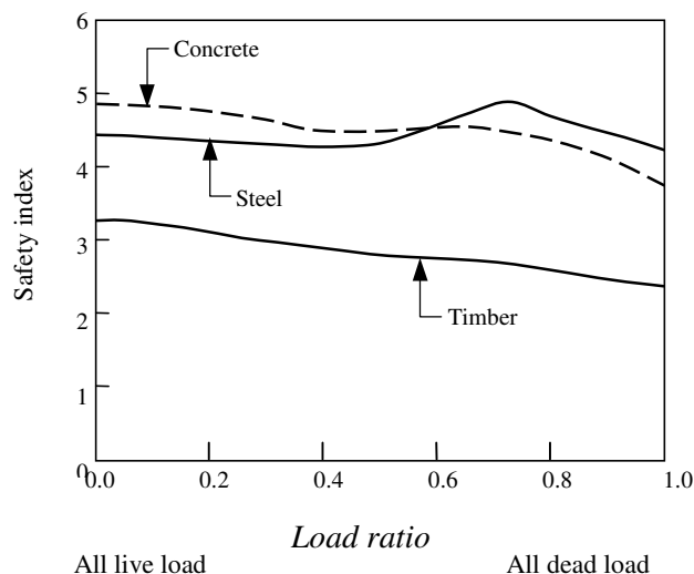
Figure 5. The computed safety of beam elements (Source: Leicester et al. 1986[24])
