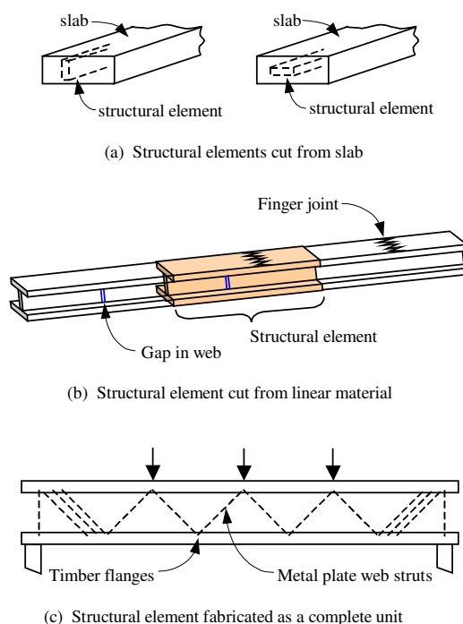
Figure 3. Examples of composite wood structural elements.
