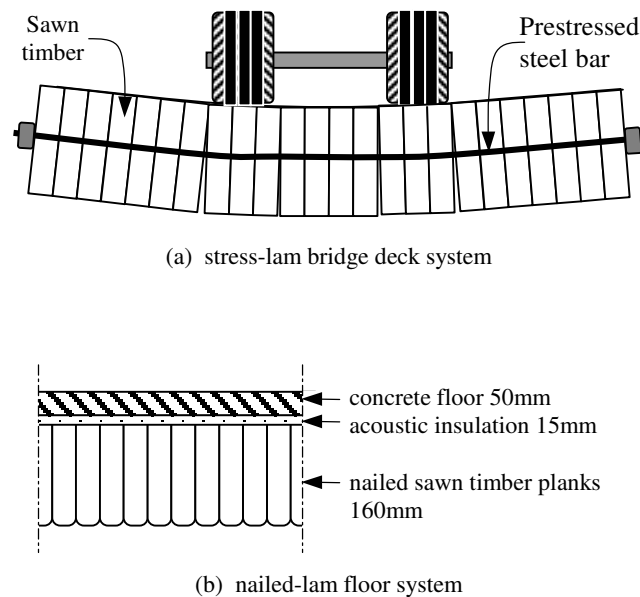
Figure 2. Examples of laminated composite systems.
