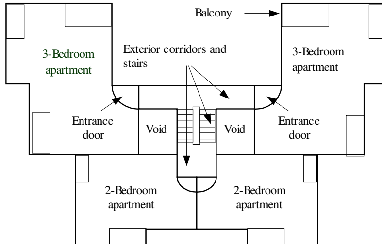
Figure 6. Plan of 3-storey apartment used for risk analysis.
