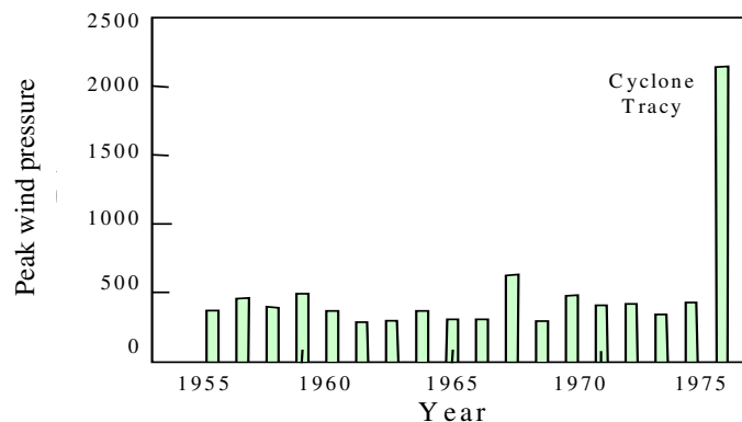
Figure 4. Annual peak wind gust pressures measured in Darwin.
